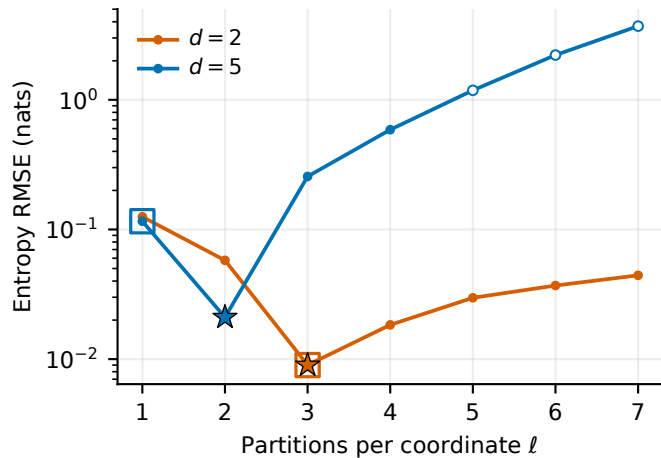
(a) Fixed n = 100,000 ; varying dimension
