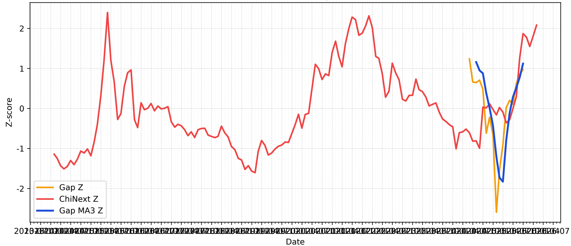
Gap vs ChiNext (Z) + Gap MA3 | 2014-01-2026-01
