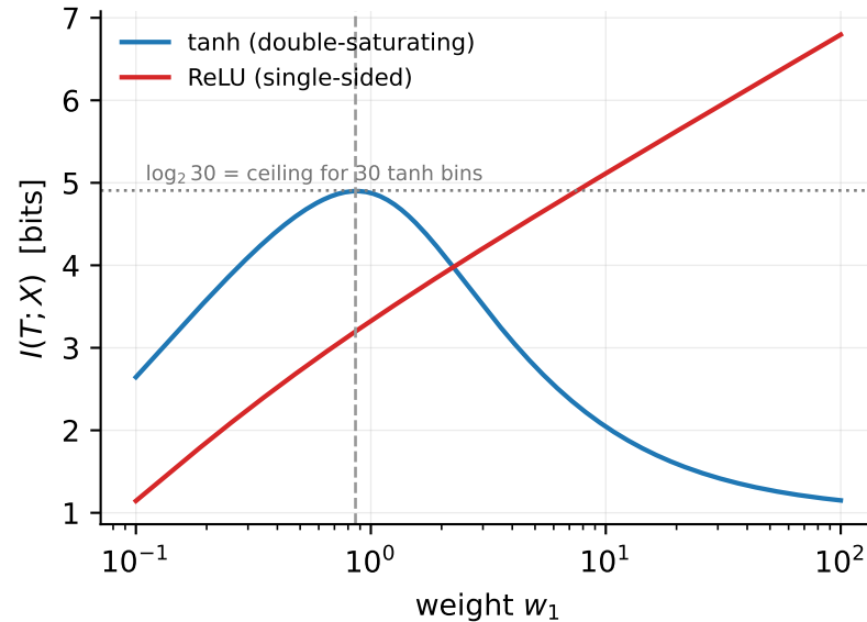
B: exact I(T; X) as the weight grows
