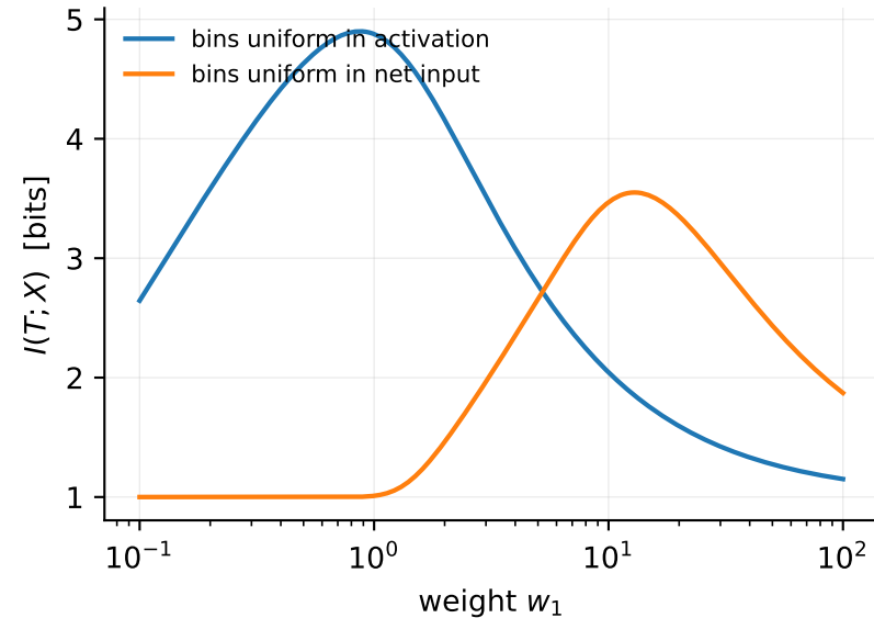
C: same network, same weights, different bin edges
