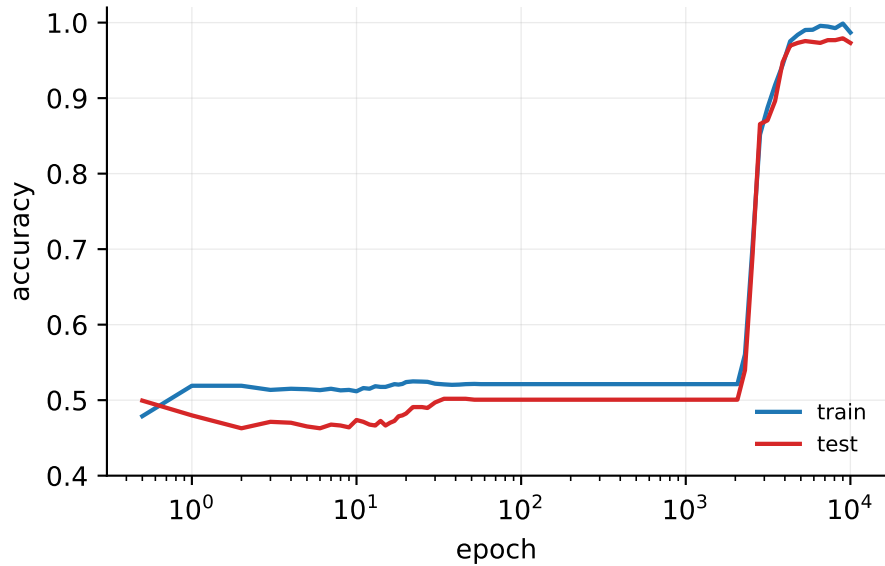
relu network
