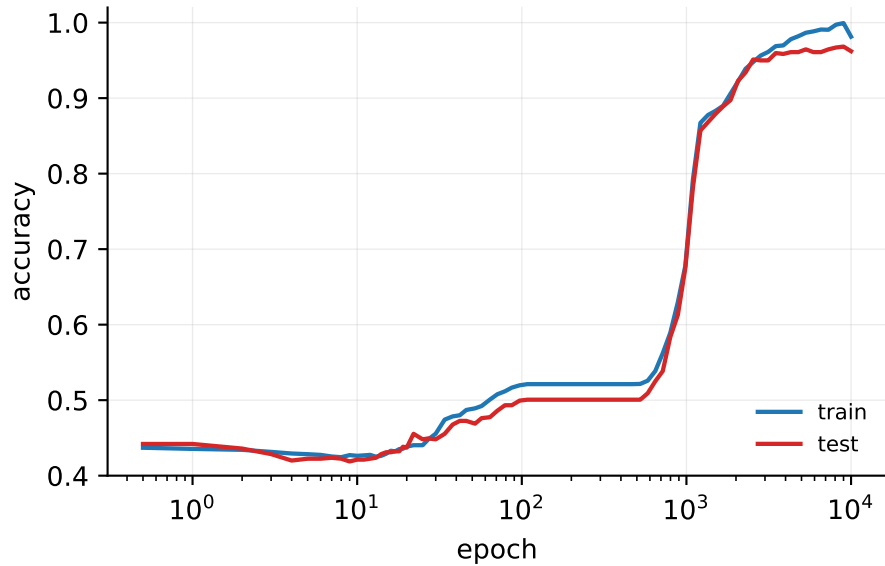
tanh network
