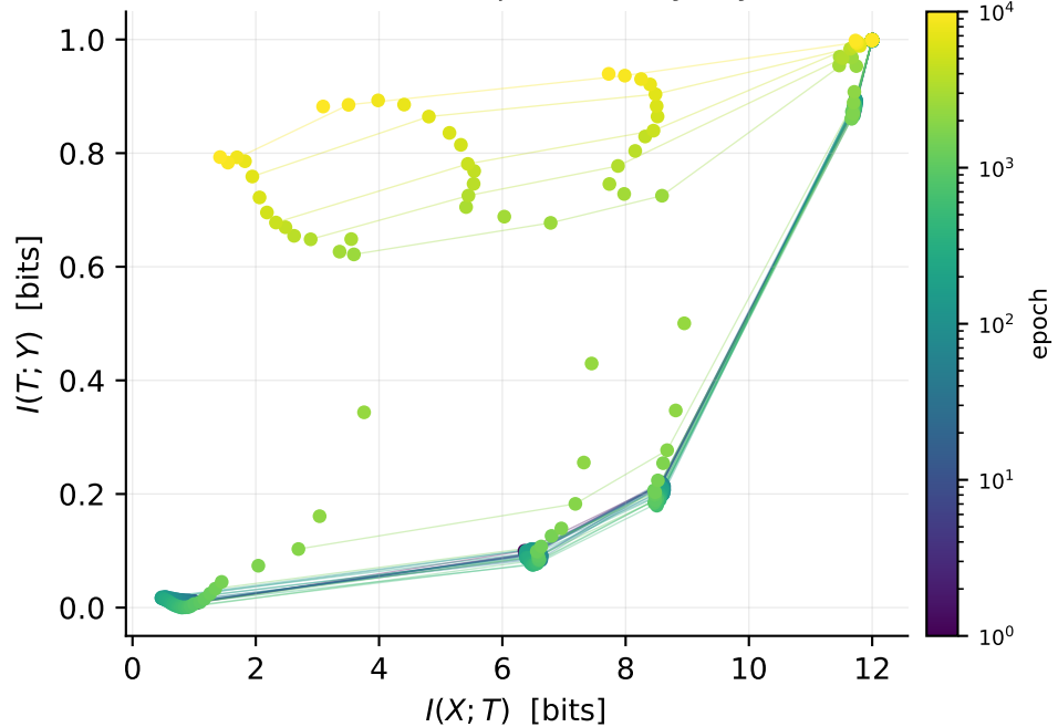
D: ...and compresses anyway
