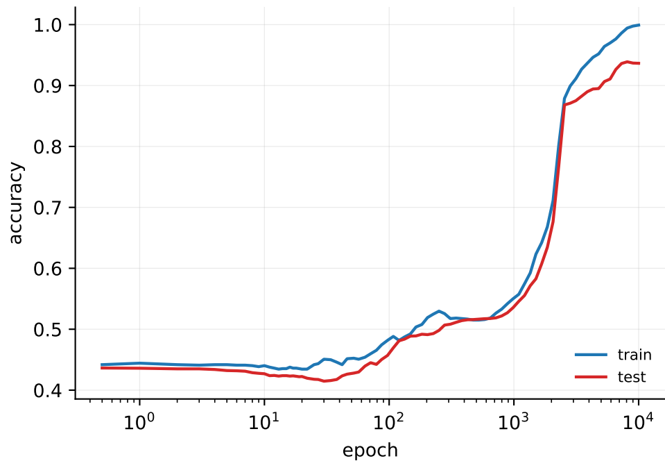
C: tanh on 30% of the data — overfits
