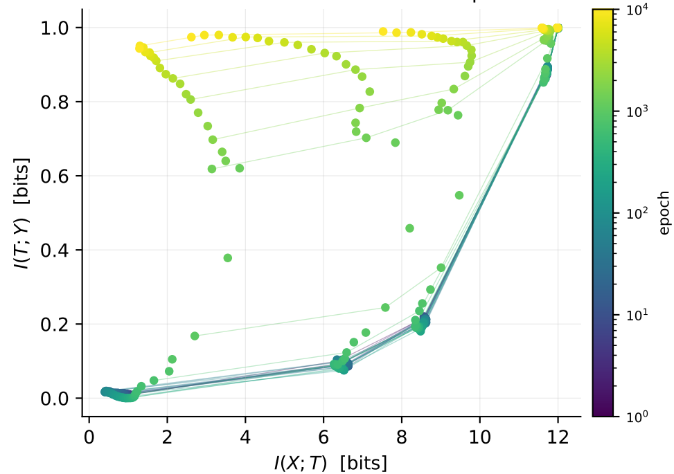
bins uniform in ACTIVATION → compression
