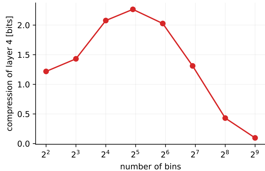
C: 'how much does it compress?' is a function of the bin count
