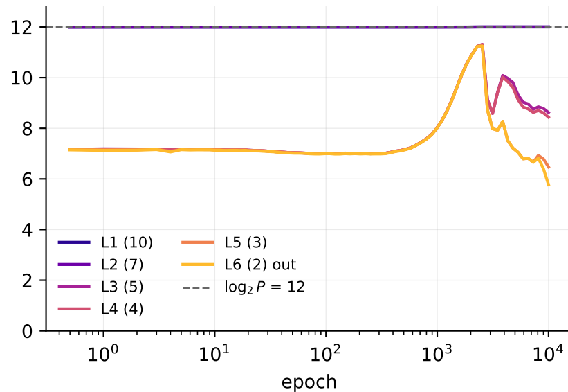
B: ReLU at machine precision
