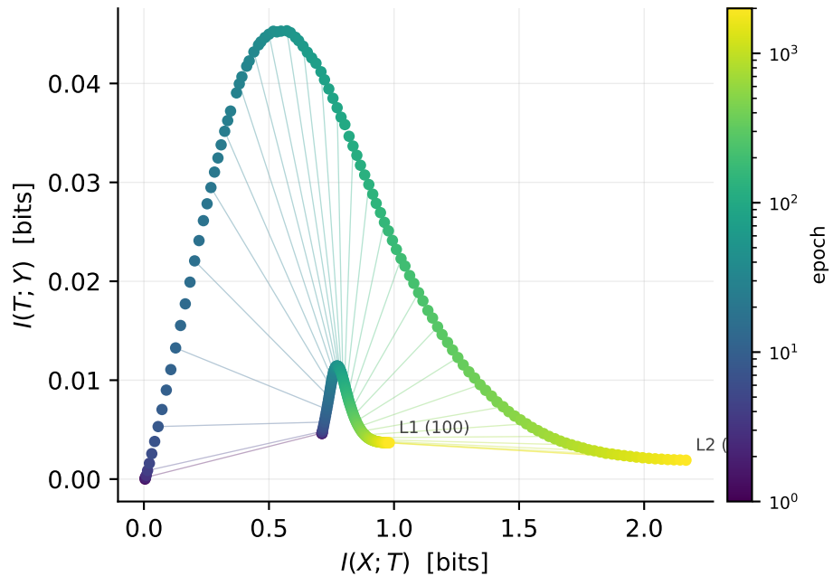
B: information plane — still no compression
