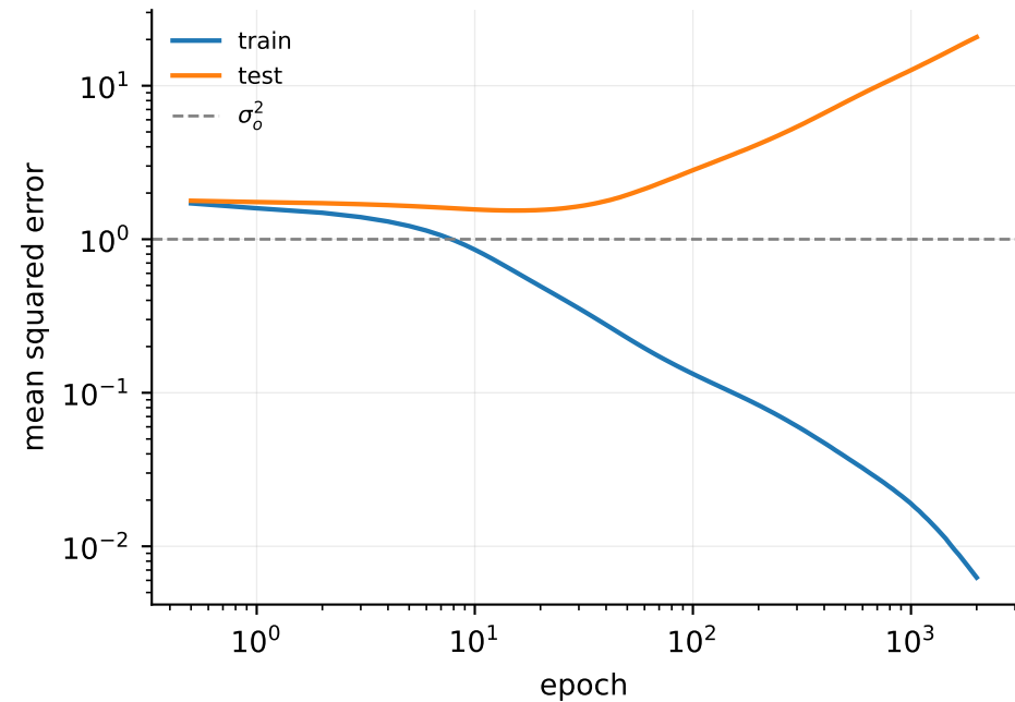
A: severe overtraining ( P = N_i , SGD)
