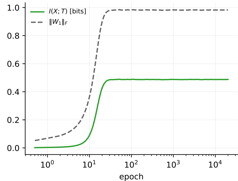
C: ...yet information only ever RISES
