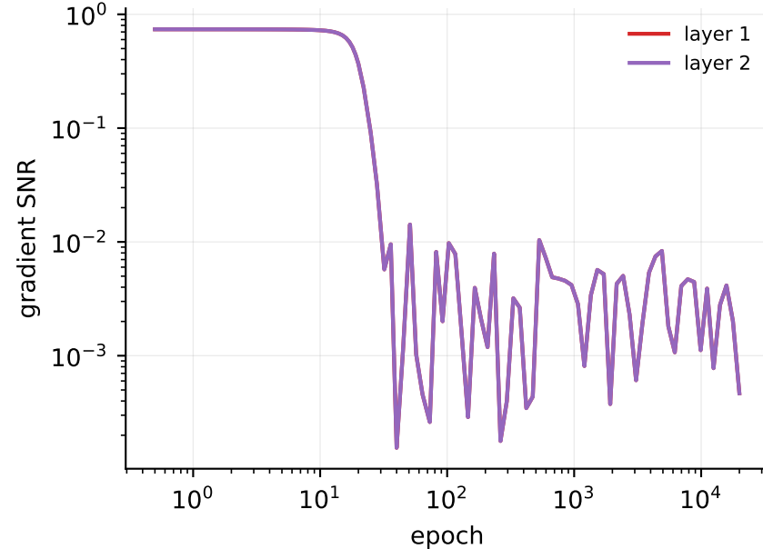
B: the drift \rightarrow diffusion transition IS present
