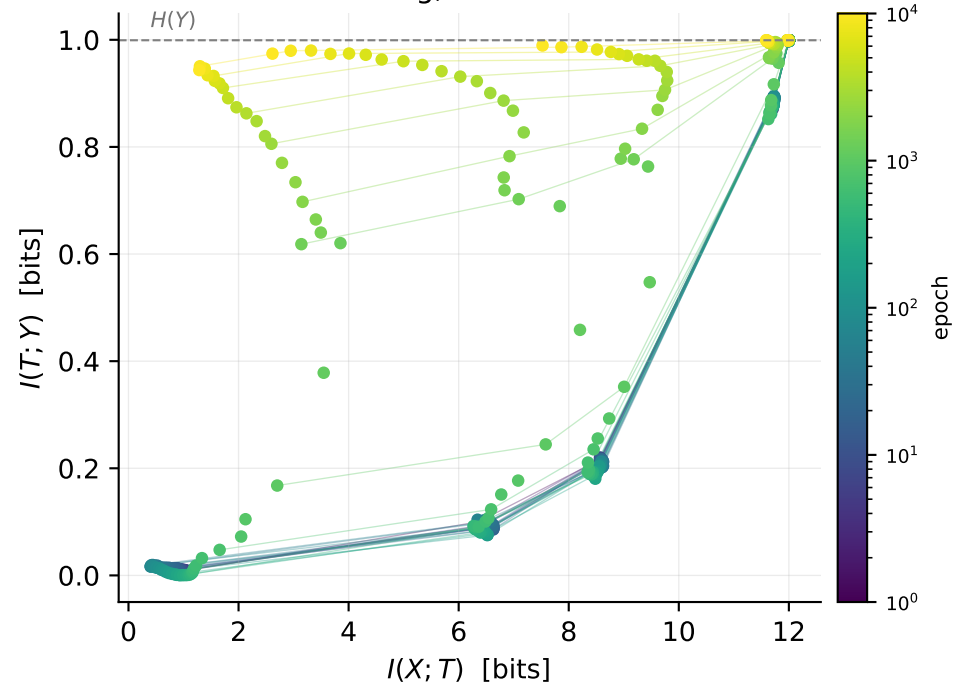
A: tanh — fitting, then COMPRESSION
