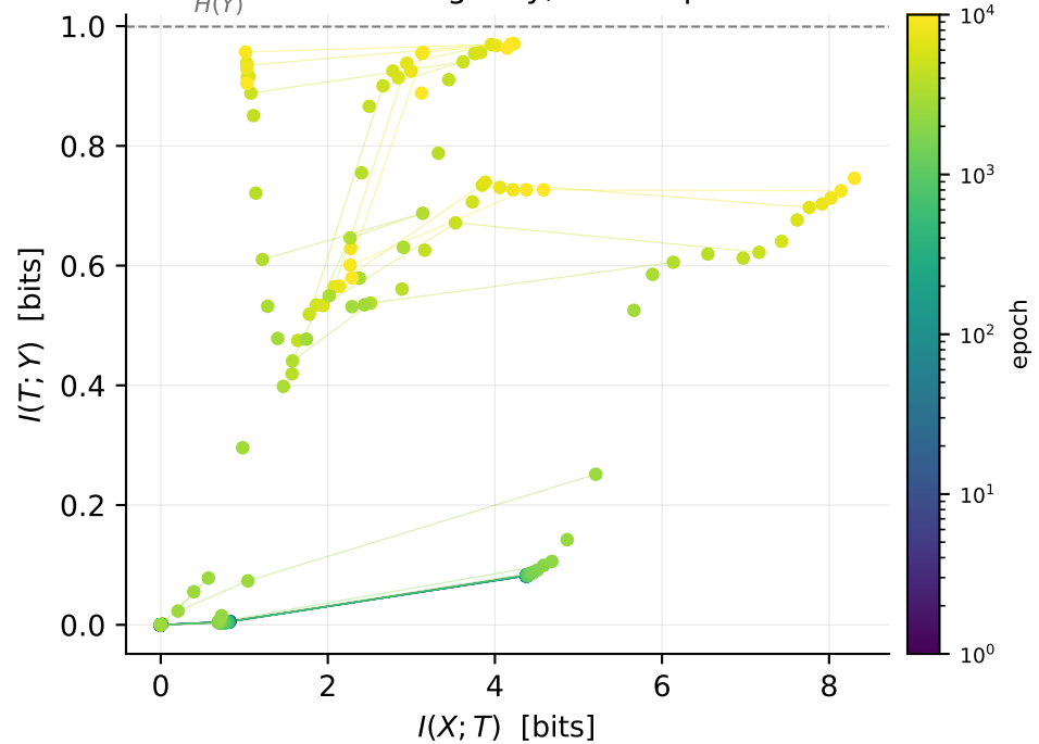
B: ReLU — fitting only, no compression
