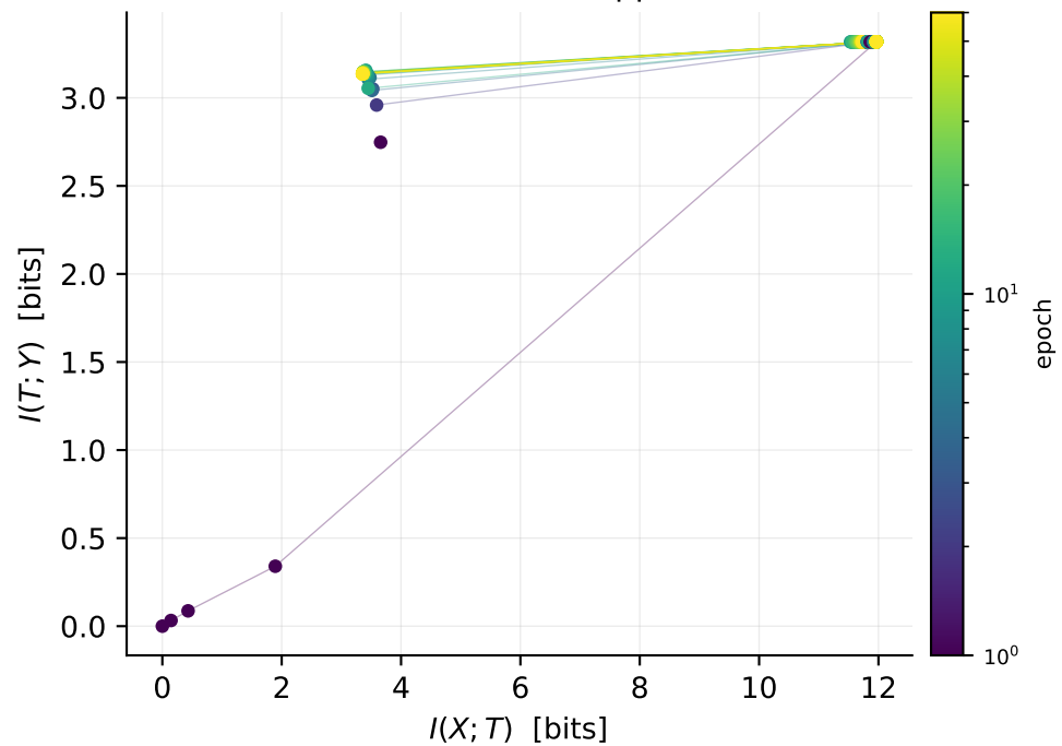
D: relu on MNIST (KDE upper bound)
