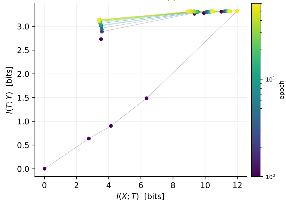
C: tanh on MNIST (KDE upper bound)
