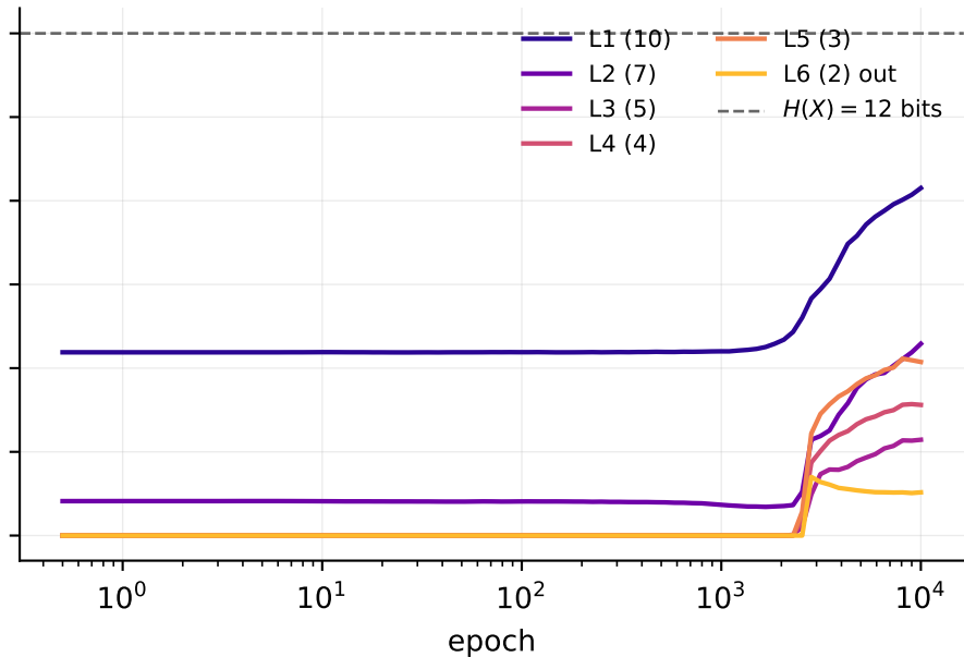
ReLU
