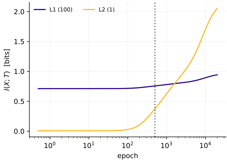
B: I(X; T) keeps increasing
