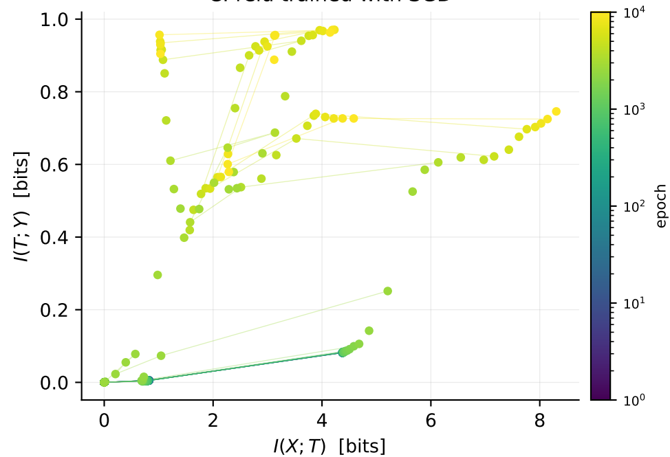
C: relu trained with SGD
