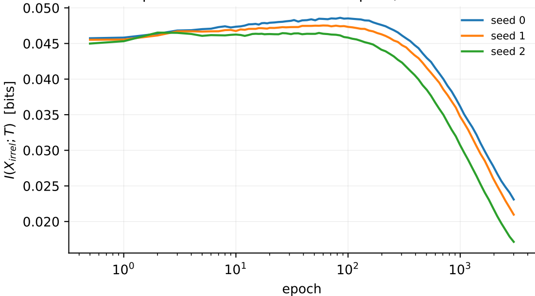
Compression of the irrelevant subspace, across seeds
