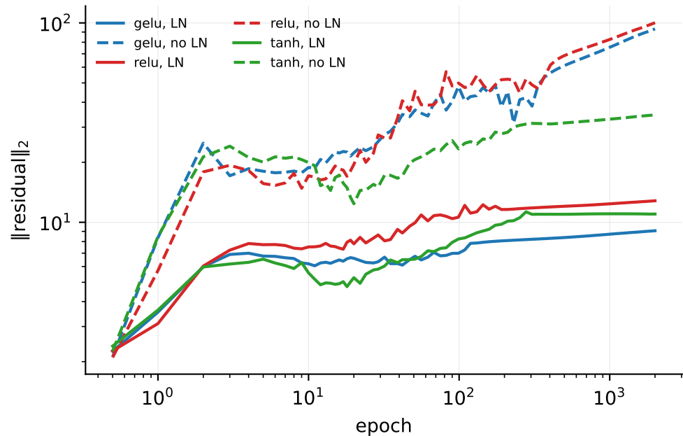
Residual stream norm (block 2)
