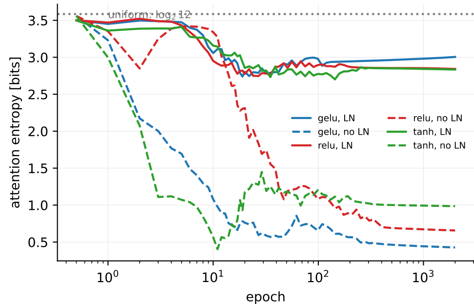
Attention sharpens (block 2)
