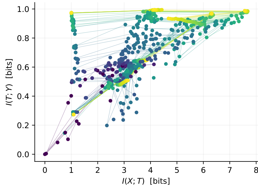
relu, NO LayerNorm
