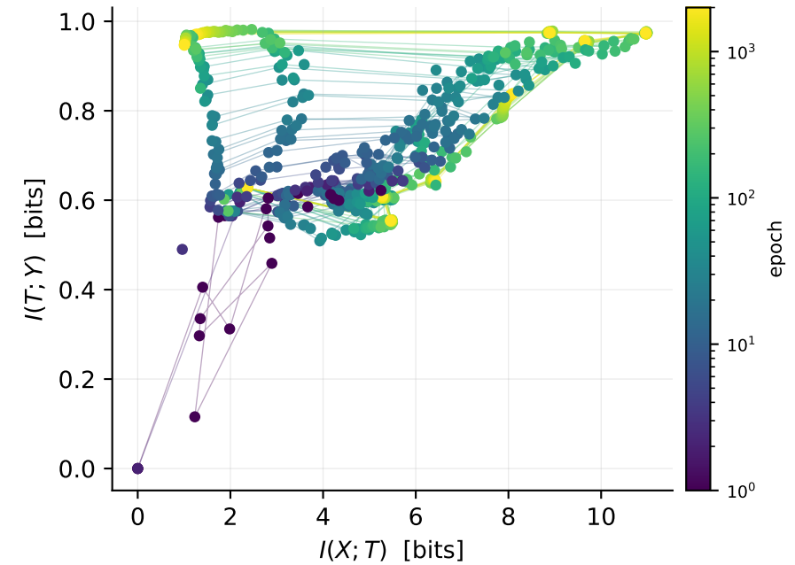
tanh, NO LayerNorm
