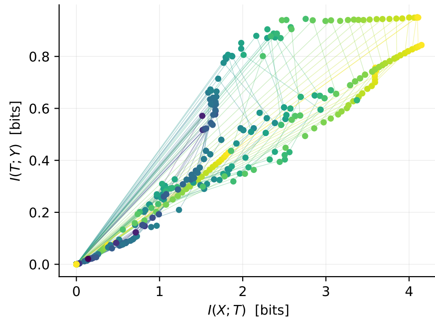
gelu, NO LayerNorm
