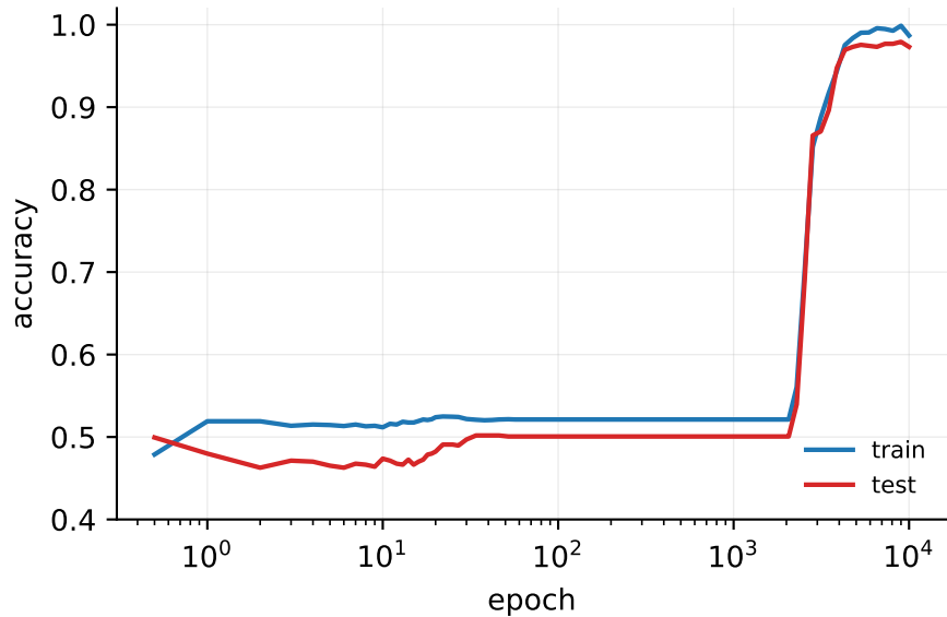
A2: relu network
