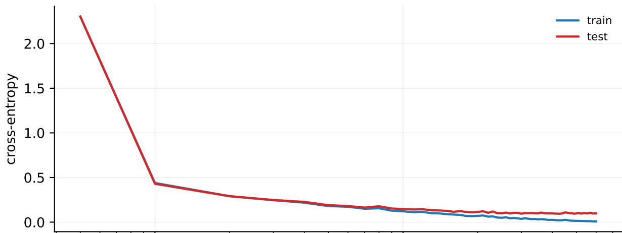
tanh on MNIST
