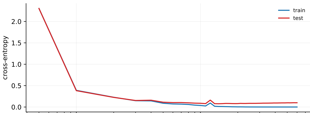
ReLU on MNIST
