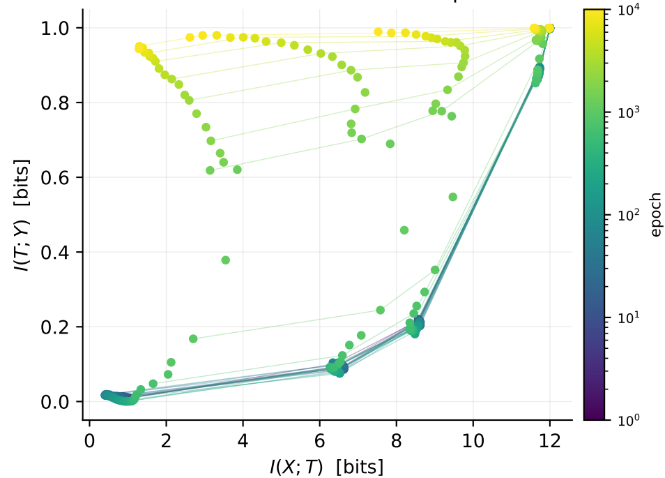
Bins uniform in activation \rightarrow compression
