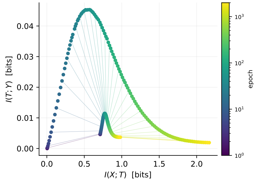
A: SGD (5 samples / batch)
