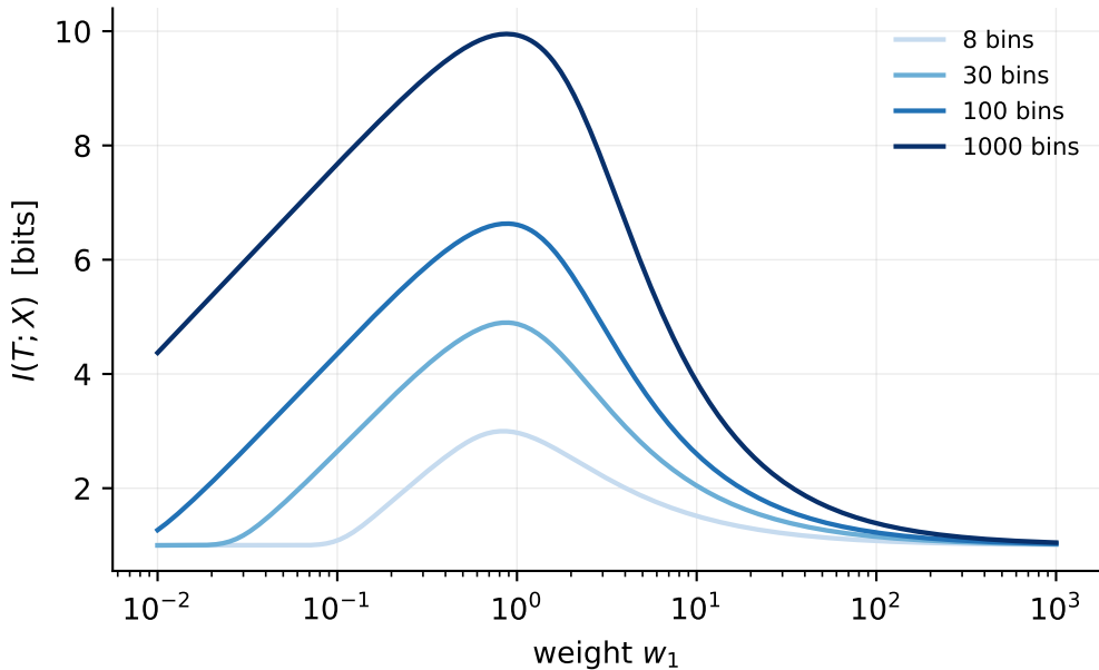
Bin count shifts the curve bodily
