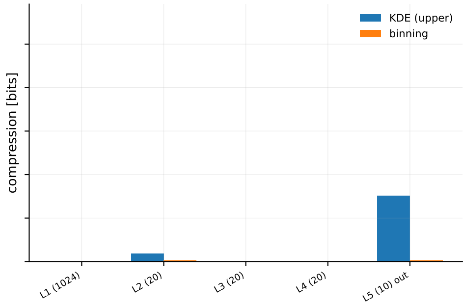
relu
