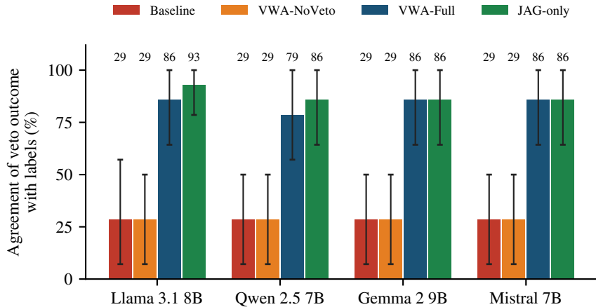
(a) Four local LLMs, T=0
