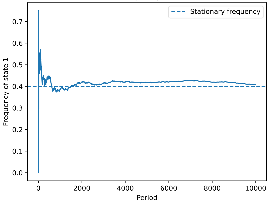
State 1 Frequency Over Time
