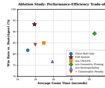
Fig. 1. Ablation Study: Performance-Efficiency Trade-off. The Full System (star) achieves the best balance between win rate and wall-clock time.
