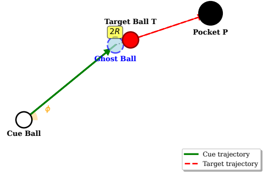
Fig. 2. Ghost Ball geometry. The cue ball aims at the virtual point G (ghost ball center) such that the line from target ball T to pocket P becomes the post-impact trajectory. The offset magnitude is 2R along the T \rightarrow P direction.
