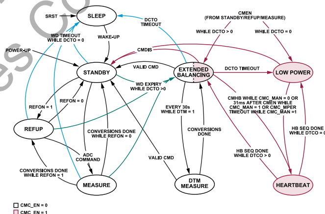
Figure 25. State Diagram with Low Power Cell Monitoring
