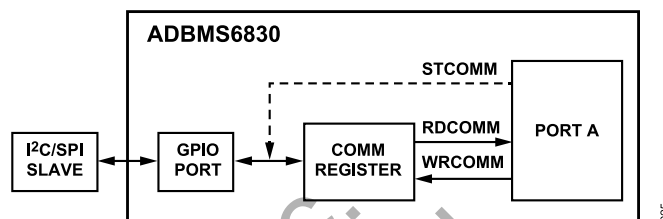
Figure 26. I 2 C/SPI Master Using GPIOs
