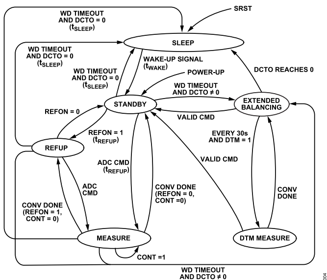
Figure 15. Core State Diagram
