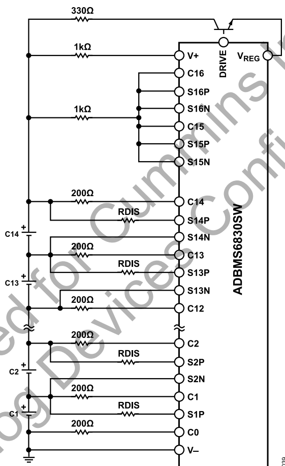
Figure 44. Cell Depopulation in LFCSP-SS Package
