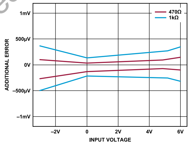
Figure 41. Cell Voltage Residual Error After Compensation
