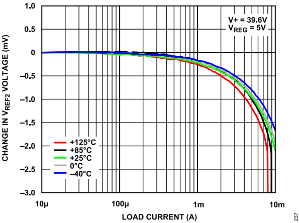
Figure 12. Change in V_{REF2} Voltage vs. Load Current
