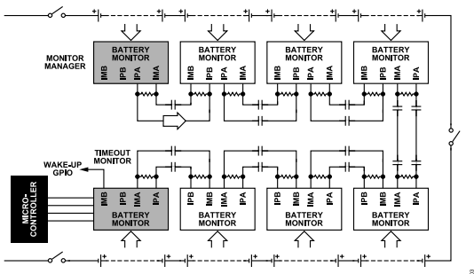
Figure 23. Bridgeless Timeout Monitor System Configuration
