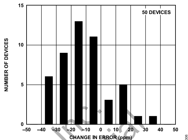
Figure 9. C-ADC Gain Error Due to IR Reflow
