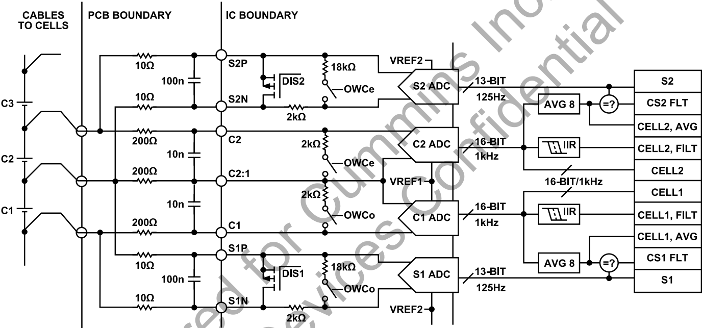
Figure 19. Open Wire Detection
