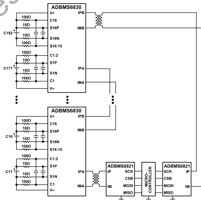
Figure 31. Multiple Devices Configured for Reversible isoSPI
