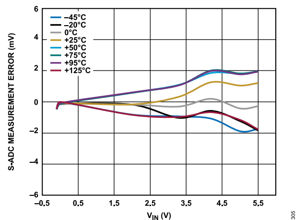
Figure 11. S-ADC Measurement Error vs. V_{IN}
