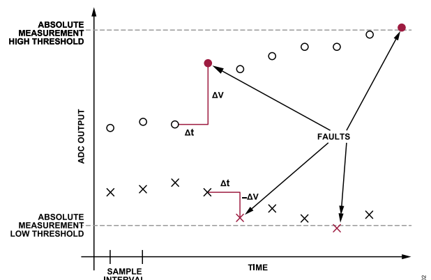
Figure 22. UV, OV, and DV Threshold Comparisons
