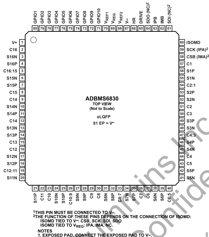
Figure 4. Pin Configuration, 80-Lead LQFP_EP
