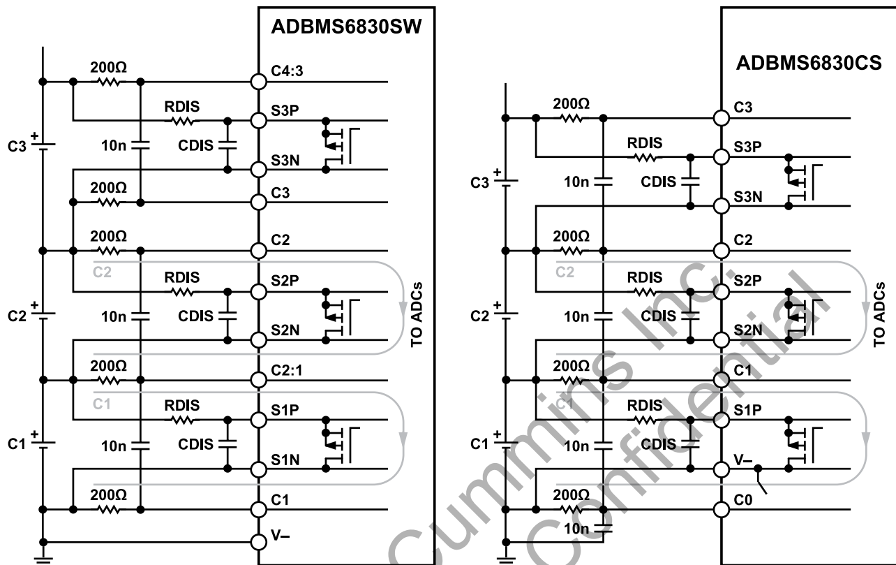
Figure 40. Input Filtering and Balancing Network
