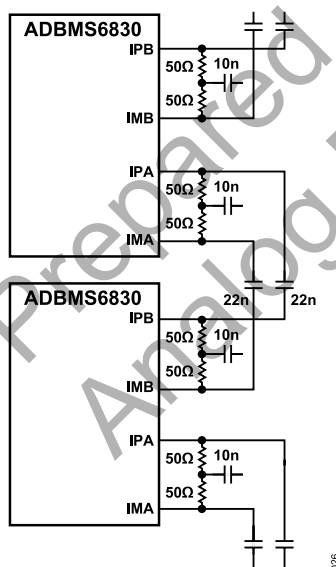
Figure 30. Capacitor Isolated isoSPI
