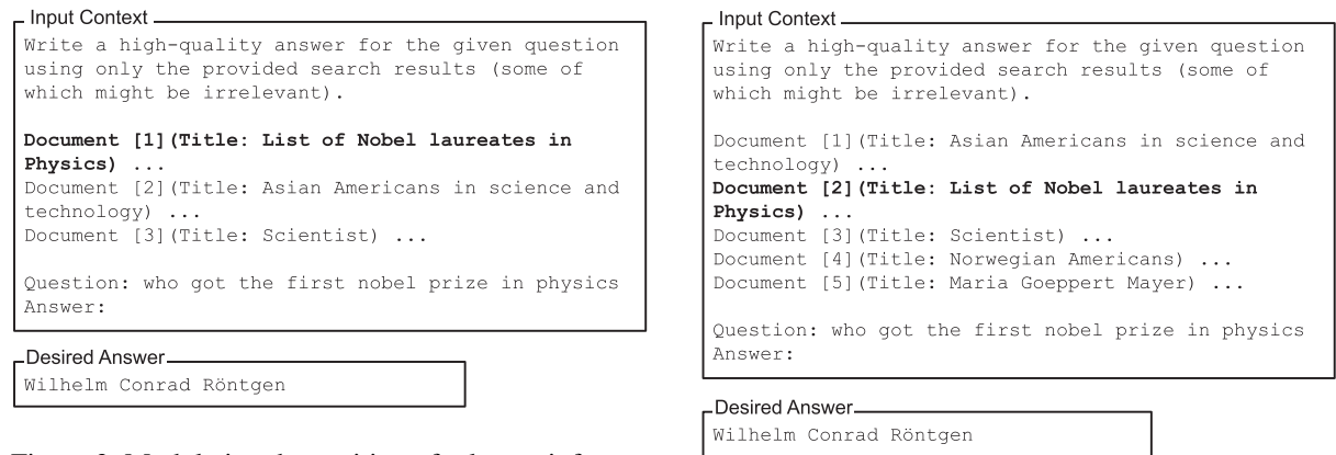
Figure 3: Modulating the position of relevant information within the input context for the multi-document question answering example presented in Figure 2. Re-ordering the documents in the input context does not affect the desired output.
