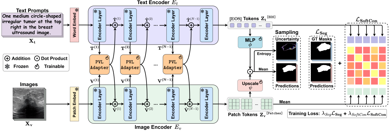
Figure 2. Overview of the proposed MedCLIPSeg framework for text-driven medical image segmentation. The model extends CLIP with vision and language encoders connected via PVL Adapters, which perform confidence-weighted image-text fusion at multiple deep layers. Segmentation and uncertainty maps arise from the mean and entropy of posterior samples, with a soft patch-level contrastive loss.
