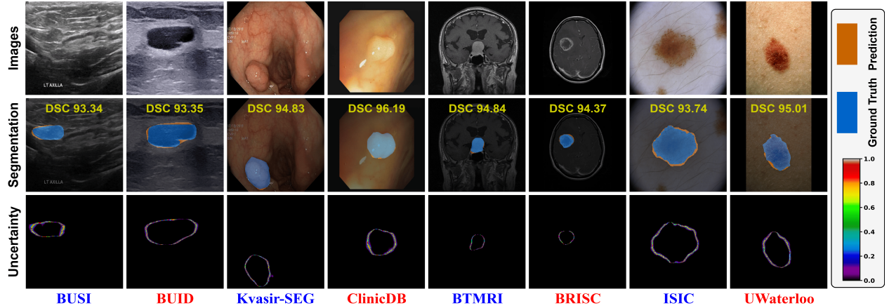
Figure 4. Segmentation and uncertainty visualizations. Uncertainty peaks along lesion boundaries and remains consistent across diverse datasets, indicating reliable calibration and generalization. ID data are in blue while OOD data are in red.
