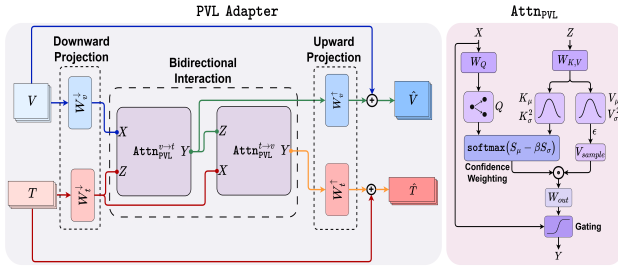
Figure 3. Illustrations of PVL Adapter and \text{Attn}_{\text{PVL}} .
