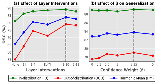
Figure 5. Layer-wise interventions ( left ) and confidence weighting ( \beta ) ( right ) ablations averaged on ID and OOD data.
