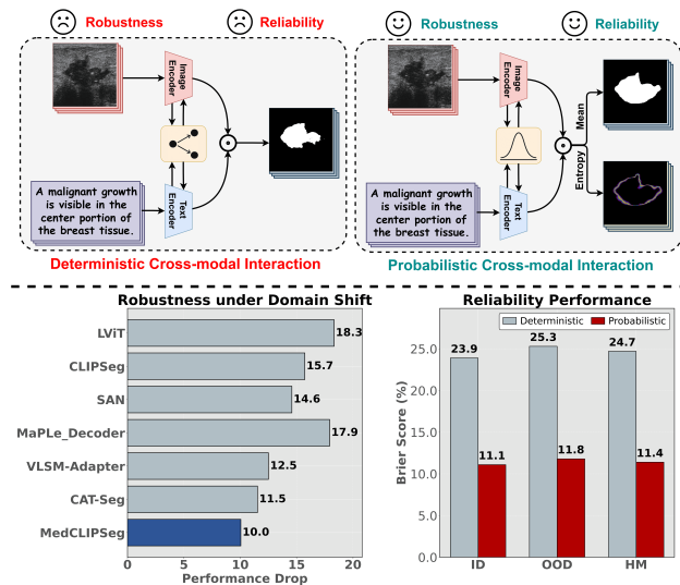
Figure 1. (Top): Comparison between deterministic and probabilistic cross-modal fusion techniques in CLIP adaptation for text-driven segmentation. Probabilistic formulation models variability in visual-textual representations as distributions, enabling more robust feature alignment. (Bottom): Robustness and Reliability plots over ID and OOD data show improved generalization, with smaller out-of-domain performance drops and better calibration of predicted confidence, reflected by lower Brier scores.
