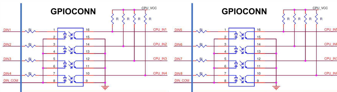
Figure 3: GPIOCONN Input Pin Schematic
