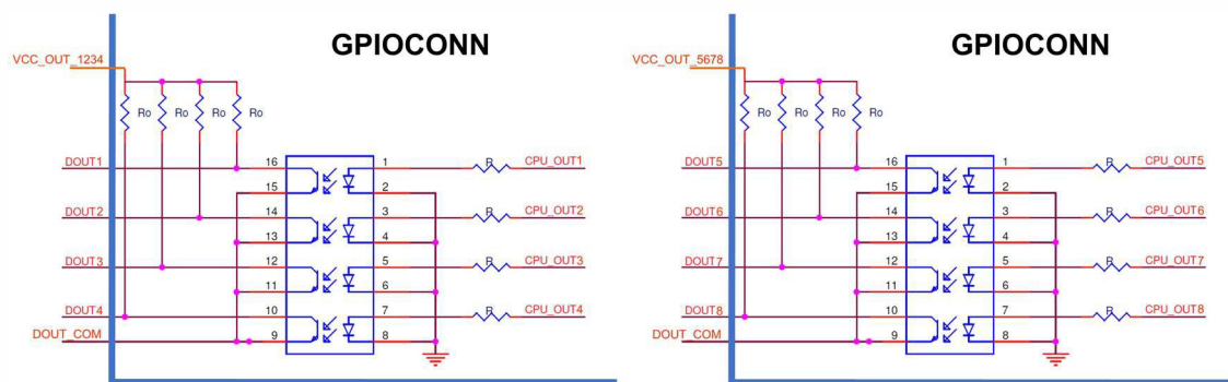
Figure 4: GPIOCONN Output Pin Schematic
