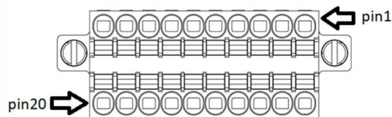
Figure 2: GPIOCONN Connector
