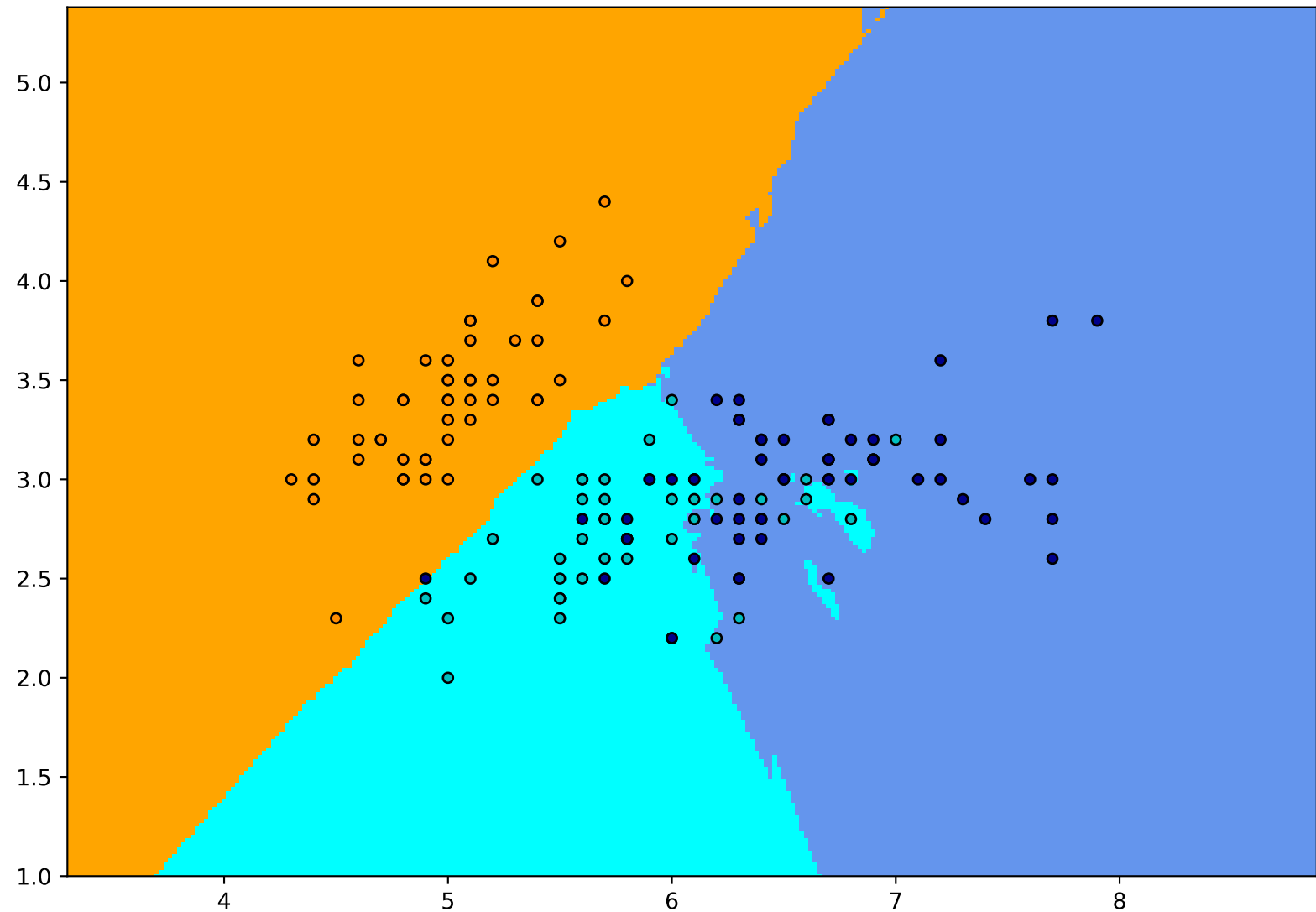
3-Class classification (k = 15, weights = 'uniform')
