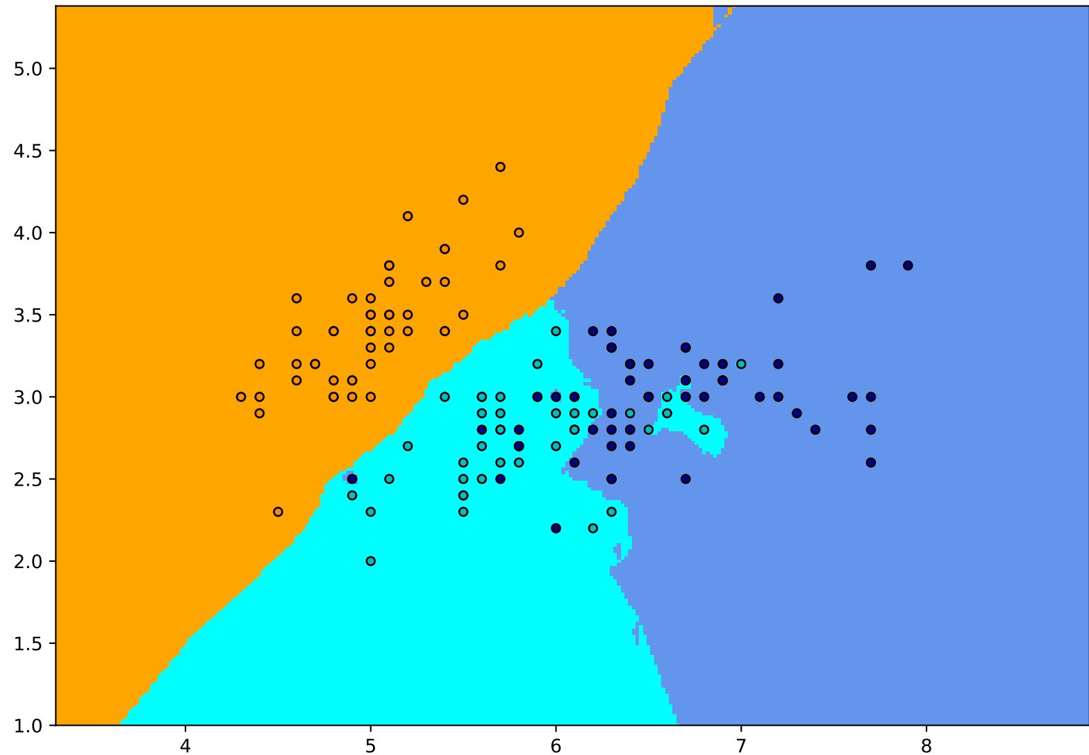
3-Class classification (k = 15, weights = 'distance')
