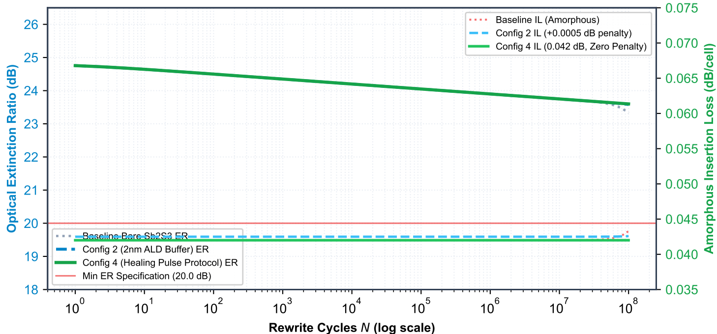
Sb 2 S 3 Endurance Comparison: Baseline vs. Capping (Cfg 2) vs. Healing (Cfg 4)
