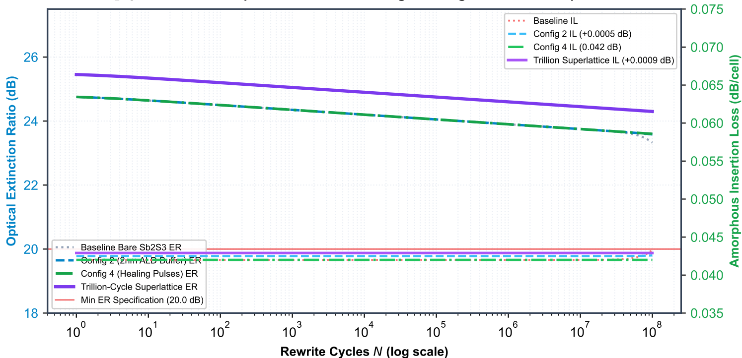
Sb 2 S 3 Endurance Comparison: Baseline vs. Cfg 2 vs. Cfg 4 vs. Trillion Superlattice
