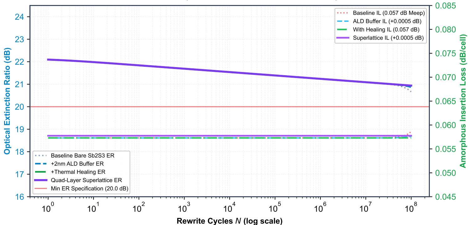
Sb 2 S 3 Endurance Comparison: Grounded in Full-Wave Meep FDTD
