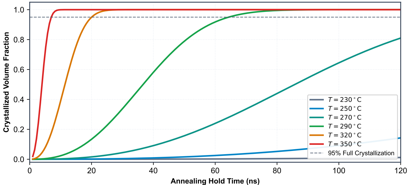
Sb 2 S 3 JMAK Crystallization Kinetics: Fraction vs. Anneal Time
