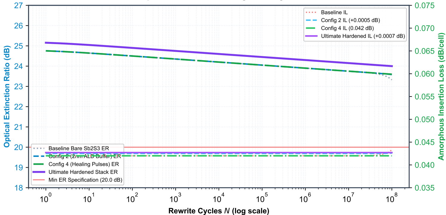
Sb 2 S 3 Endurance Comparison: Baseline vs. Cfg 2 vs. Cfg 4 vs. Ultimate Hardened
