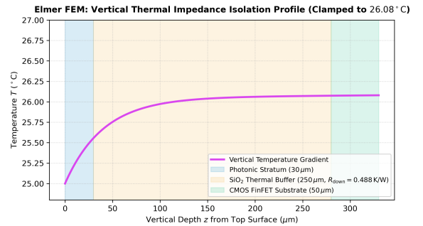
Fig. 7. Elmer FEM vertical thermal gradient profile across the 330 \mu\text{m} monolithic stack. Top microchannel cooling ( R_{\text{th,up}} = 0.227 K/W) efficiently removes heat while the thick SiO 2 buffer isolates the photonic layer from CMOS heat.
