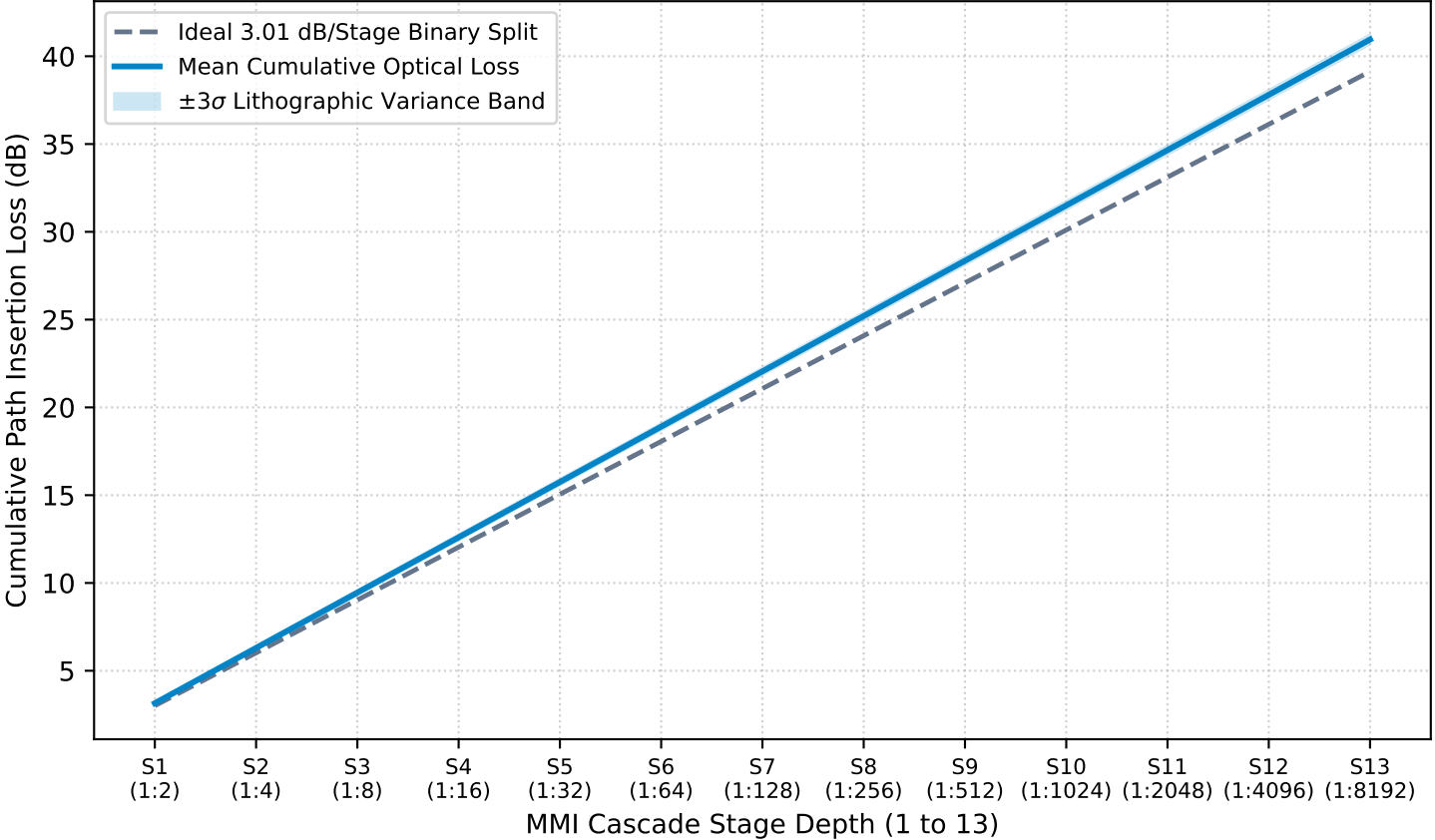
13-Stage Cascaded MMI Optical Distribution Tree: Cumulative Loss Progression
