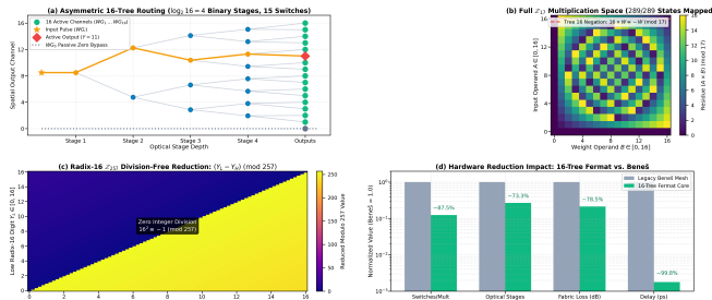
Fig. 5. Architectural formalization of the Asymmetric 16-Tree Fermat Core. (a) 4-stage binary tree routing fabric ( \log_2 16 = 4 ) with 17-channel spatial alphabet ( WG_0 \dots WG_{16} ). (b) Complete \mathbb{Z}_{17} multiplication residue space (289/289 states mapped, 100% state efficiency) and Tree 16 negation symmetry ( 16 \times W \equiv -W \pmod{17} ). (c) Radix-16 \mathbb{Z}_{257} division-free modular reduction: ( Y_L - Y_H ) ( \pmod{257} ). (d) Hardware complexity and loss scaling metrics (240 switches/multiplier, 4 cascaded stages, 1.61 dB fabric loss).
