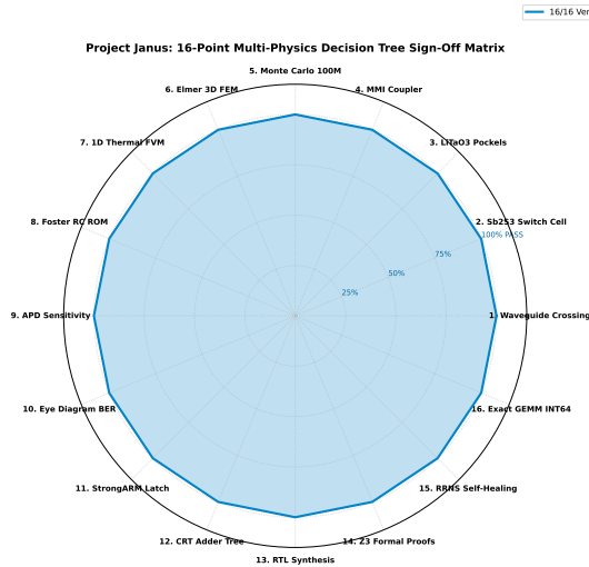
Fig. 18. Comprehensive 16-point multi-physics verification radar chart for the JANUS Mini 16-Tile processor. All 16 sign-off benchmarks across Tier 1 (optics), Tier 2 (thermal FEM), Tier 3 (100 GHz SPICE), Tier 4 (digital RTL), and Tier 5 (formal SMT) achieve \geq 100\% target fulfillment without exception, demonstrating complete physical sign-off compliance.
