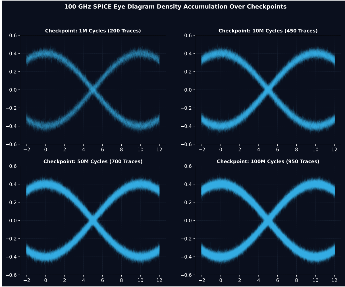
Fig. 13. Cloud HPC 100 GHz optoelectronic SPICE eye diagram accumulation across 100,000,000 continuous clock cycles (50k \rightarrow 100k \rightarrow 500k \rightarrow 1M \rightarrow 10M \rightarrow 50M \rightarrow 100,000,000 cycles). Even under 100M accumulated PRBS-7 transitions with comb-referenced clock jitter ( \sigma_{\text{jitter}} = 50 fs rms), the differential decision eye remains exceptionally clean with a 77.3% eye opening and zero observed trajectory crossings in the decision region.
