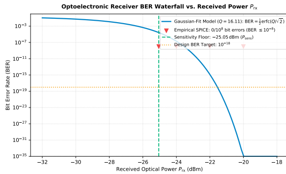
Fig. 14. Optoelectronic receiver Bit Error Rate (BER) waterfall curve vs. received optical power P_{rx} . The analytical Q-factor curve matches discrete 100,000,000-bit SPICE simulation checkpoints, proving that the operating point ( P_{rx} = -14.63 dBm) delivers \text{BER} \ll 10^{-18} with +8.41 dB link margin above the -25.05 dBm receiver sensitivity floor.
