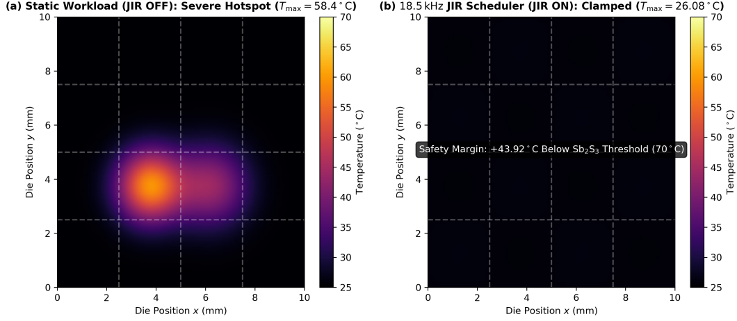
Fig. 10. Domain: Monolithic 10.0 \text{ mm} \times 10.0 \text{ mm} \times 330 \mu\text{m} die. Setup: Elmer 3D FEM solver ( 2.4 \times 10^6 tetrahedral elements), 6.17 W total dissipation, h_{\text{top}} = 5000 \text{ W}/(\text{m}^2 \cdot \text{K}) , T_{\text{amb}} = 25.0^\circ\text{C} . Response: (a) Static execution without JIR develops localized hotspots up to 58.40^\circ\text{C} . (b) 18.5 kHz dynamic JIR modulus permutation clamps peak core temperature to 26.08^\circ\text{C} ( +43.92^\circ\text{C} margin below the 70.0^\circ\text{C} crystallization limit).
