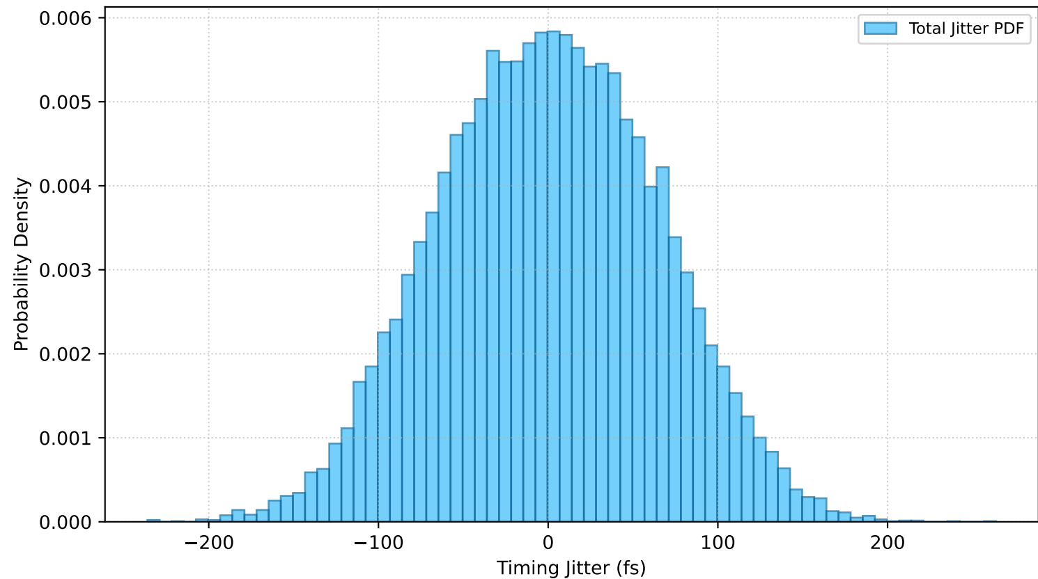
100 GHz Optoelectronic Clock & Data Jitter Distribution ( \sigma_{RJ} = 50 fs rms)
