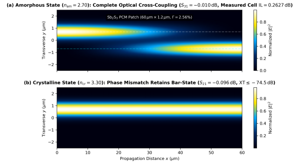
Fig. 2. MEEP 3D FDTD electromagnetic wave propagation across the optimized Sb 2 S 3 2 \times 2 directional coupler switch cell at \lambda = 1064 nm ( L = 60.0 \mu\text{m} , \Gamma = 2.56\% ). (a) Amorphous state ( n_a = 2.70 ) achieving cross-port power transfer ( S_{31} = -0.010 dB). (b) Crystalline state ( n_c = 3.30 ) phase de-coupling preserving the bar-state ( S_{21} = -0.096 dB, XT \leq -74.5 dB).
