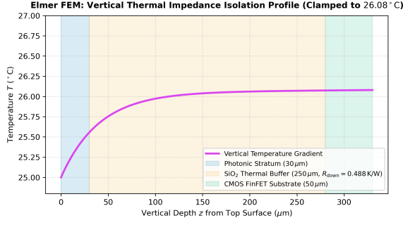
Fig. 6. Elmer FEM vertical thermal gradient profile across the 330\ \mu\text{m} monolithic stack. Top microchannel cooling ( R_{\text{th,up}} = 0.227\ \text{K/W} ) efficiently removes heat while the thick \text{SiO}_2 buffer isolates the photonic layer from CMOS heat.
