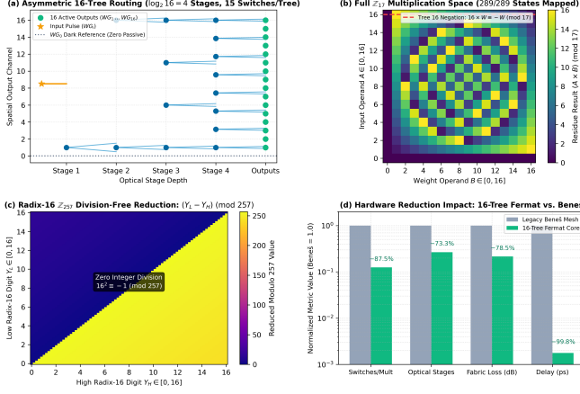
Fig. 4. Architectural formalization of the Asymmetric 16-Tree Fermat Core. (a) 4-stage binary tree routing fabric ( \log_2 16 = 4 ) with 17-channel spatial alphabet ( WG_0 \dots WG_{16} ). (b) Complete \mathbb{Z}_{17} multiplication residue space (289/289 states mapped, 100% state efficiency) and Tree 16 negation symmetry ( 16 \times W \equiv -W \pmod{17} ). (c) Radix-16 \mathbb{Z}_{257} division-free modular reduction: (Y_L - Y_H) \pmod{257} . (d) Hardware complexity and loss scaling metrics (240 switches/multiplier, 4 cascaded stages, 1.61 dB fabric loss).
