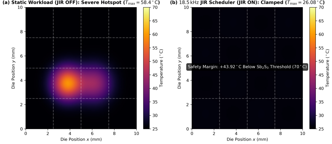
Fig. 9. Elmer FEM 3D surface temperature distributions across the JANUS Mini 16-Tile monolithic die (10.0 mm \times 10.0 mm). (a) Without JIR, localized active tiles develop severe hotspots up to 58.4°C. (b) With 18.5 kHz JIR dynamic spatial modulus rotation, peak temperature is clamped to 26.08°C, providing a +43.92°C safety margin below the 70°C phase-change crystallization threshold.
