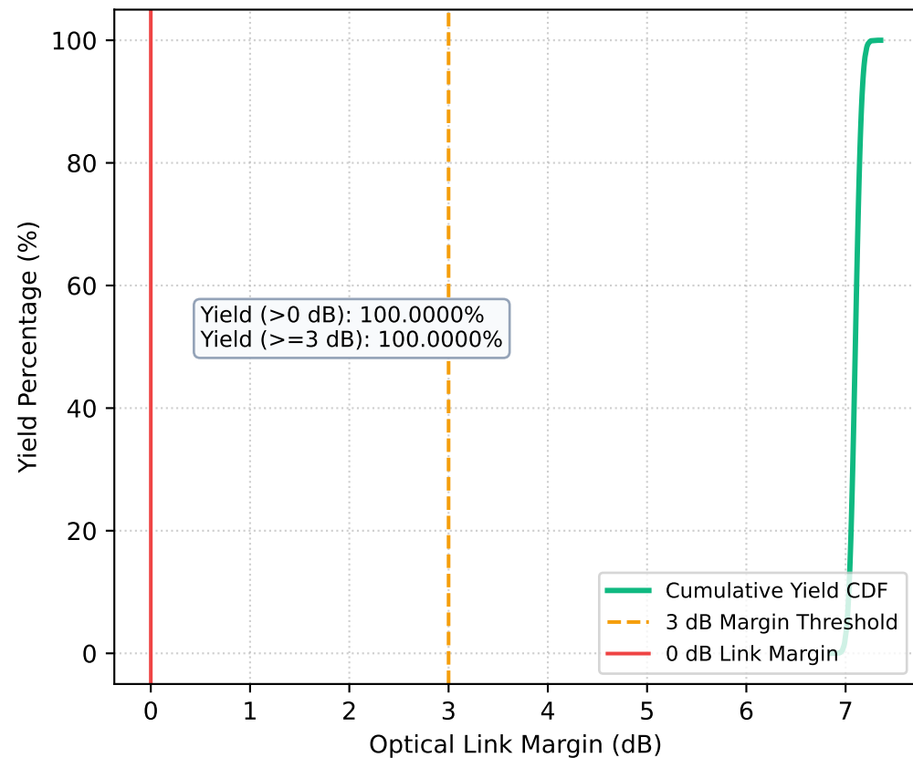
(a) Optical Link Yield CDF
