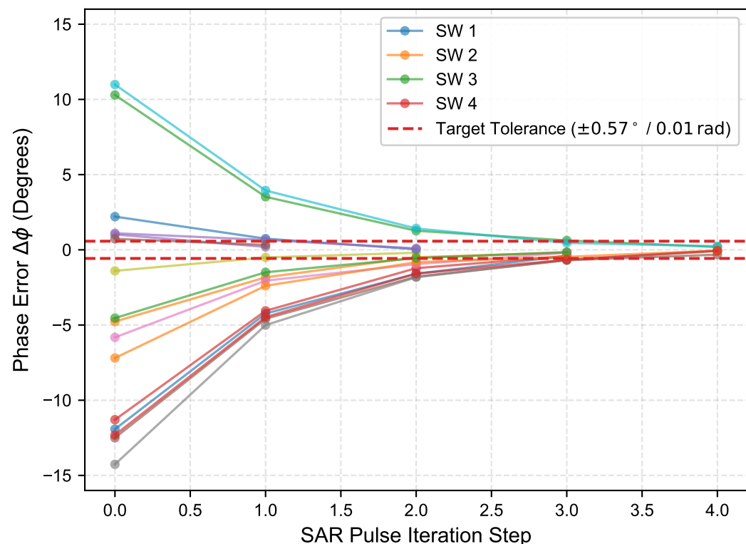
(b) Sb2S3 PCM Closed-Loop Phase Calibration All 16 Switches Converged | Max Error: 0.0073 rad | Settle Time: 1.40 \mu s
