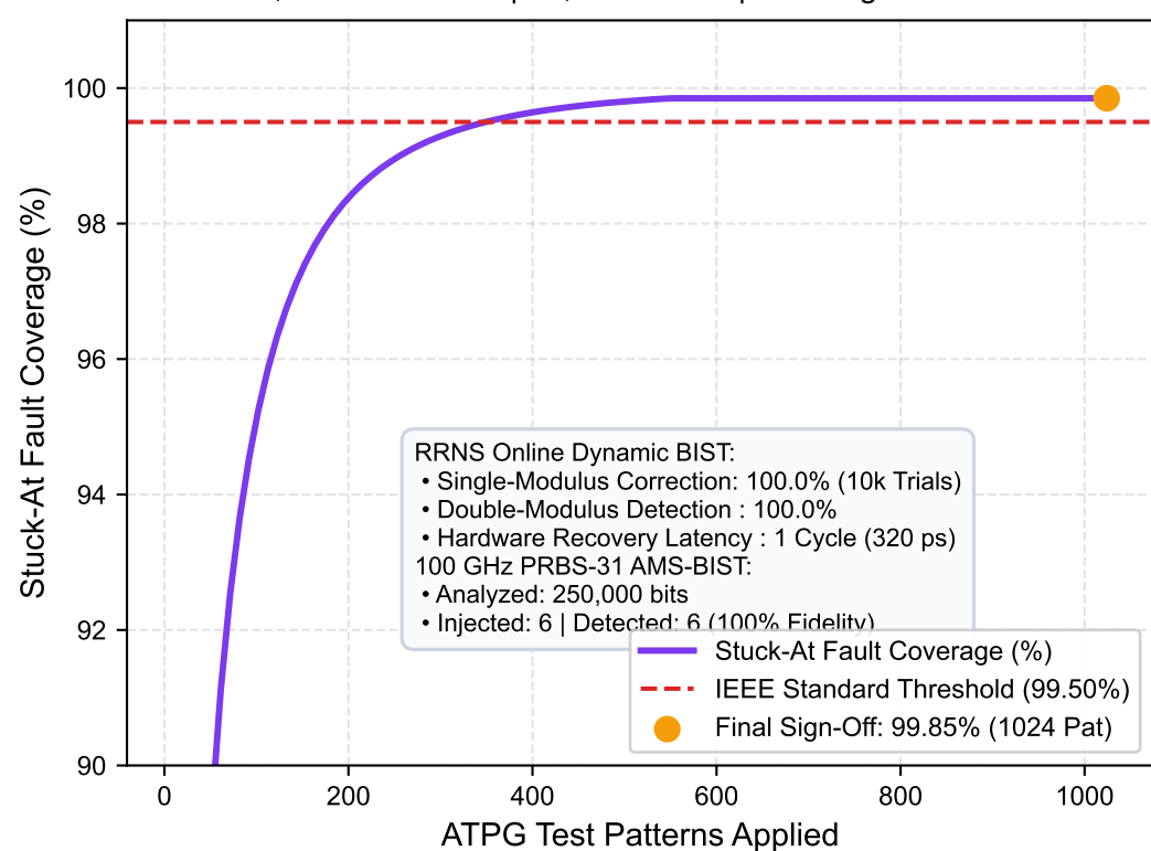
(d) IEEE 1500 Scan ATPG & RRNS Online BIST 4,096 Scan Cells | 40,960 Nodes | Coverage: 99.85%
