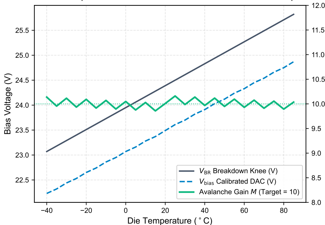
(c) Dynamic APD Bias Tracking DAC (-40 C to +85 C) Fixed Multiplication Gain M = 10.0 \pm 0.16 Across Thermal Envelope
