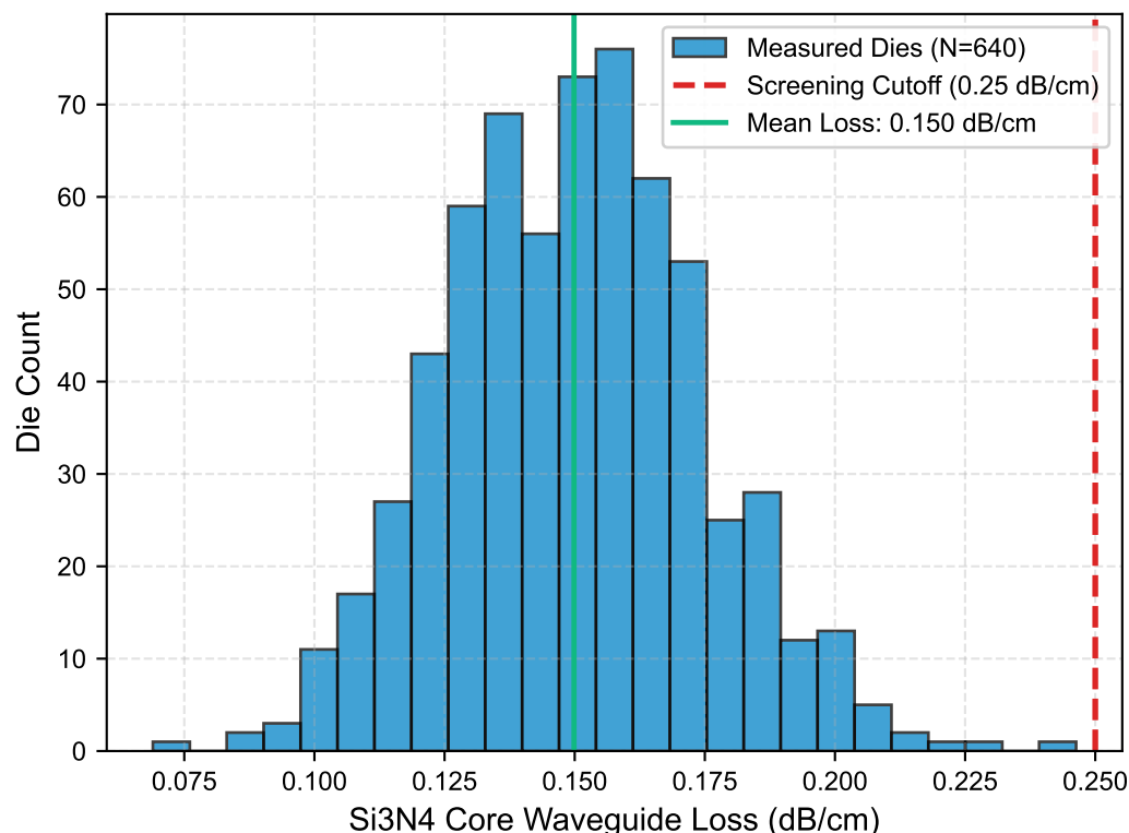
(a) Wafer-Level Optical Loopback Screening (P-BIST) Yield: 100.0% (640/640 Passed) | Grating Coupler: 2.12 dB
