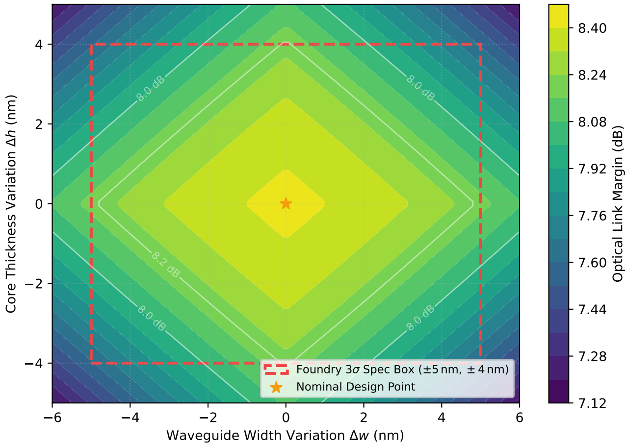
2D Manufacturing Process Window: Optical Link Margin vs. ( \Delta w, \Delta h )
