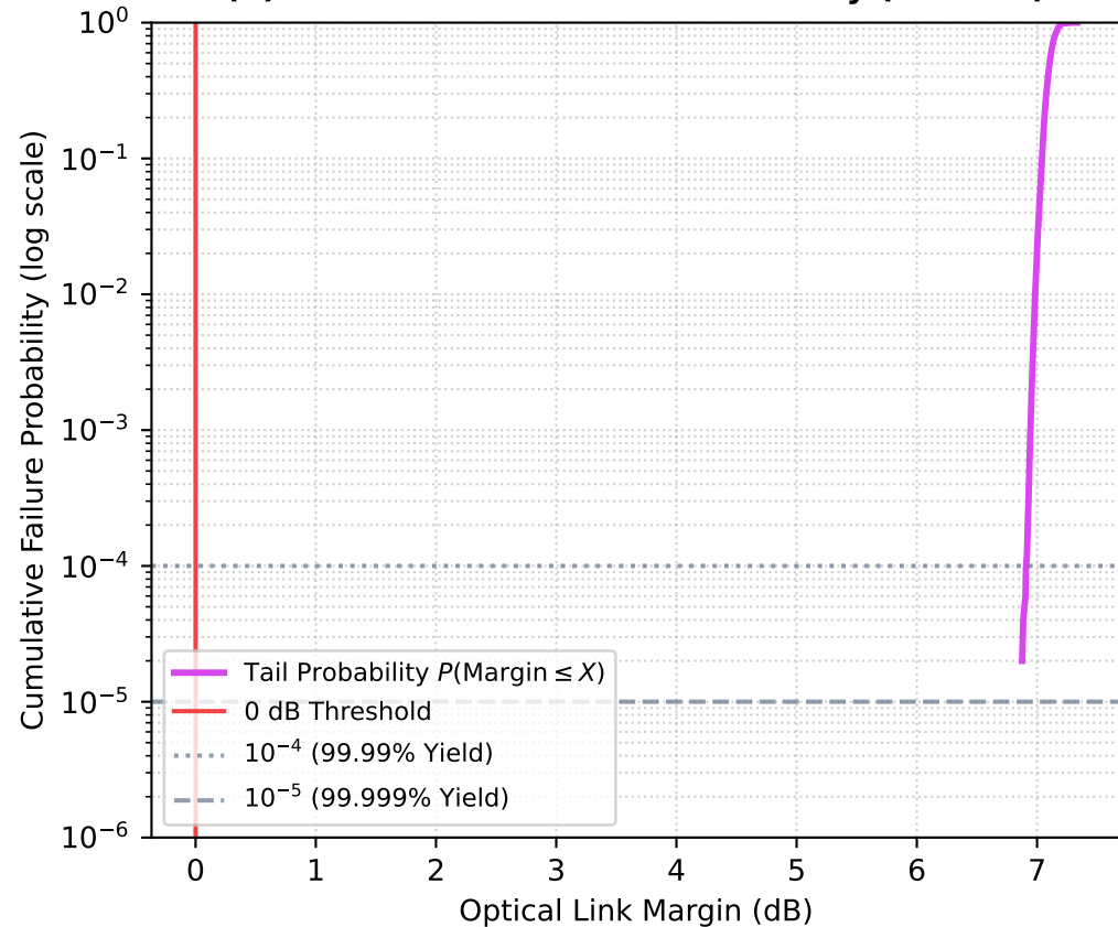
(b) Extreme Tail Failure Probability ( 1 - \text{Yield} )
